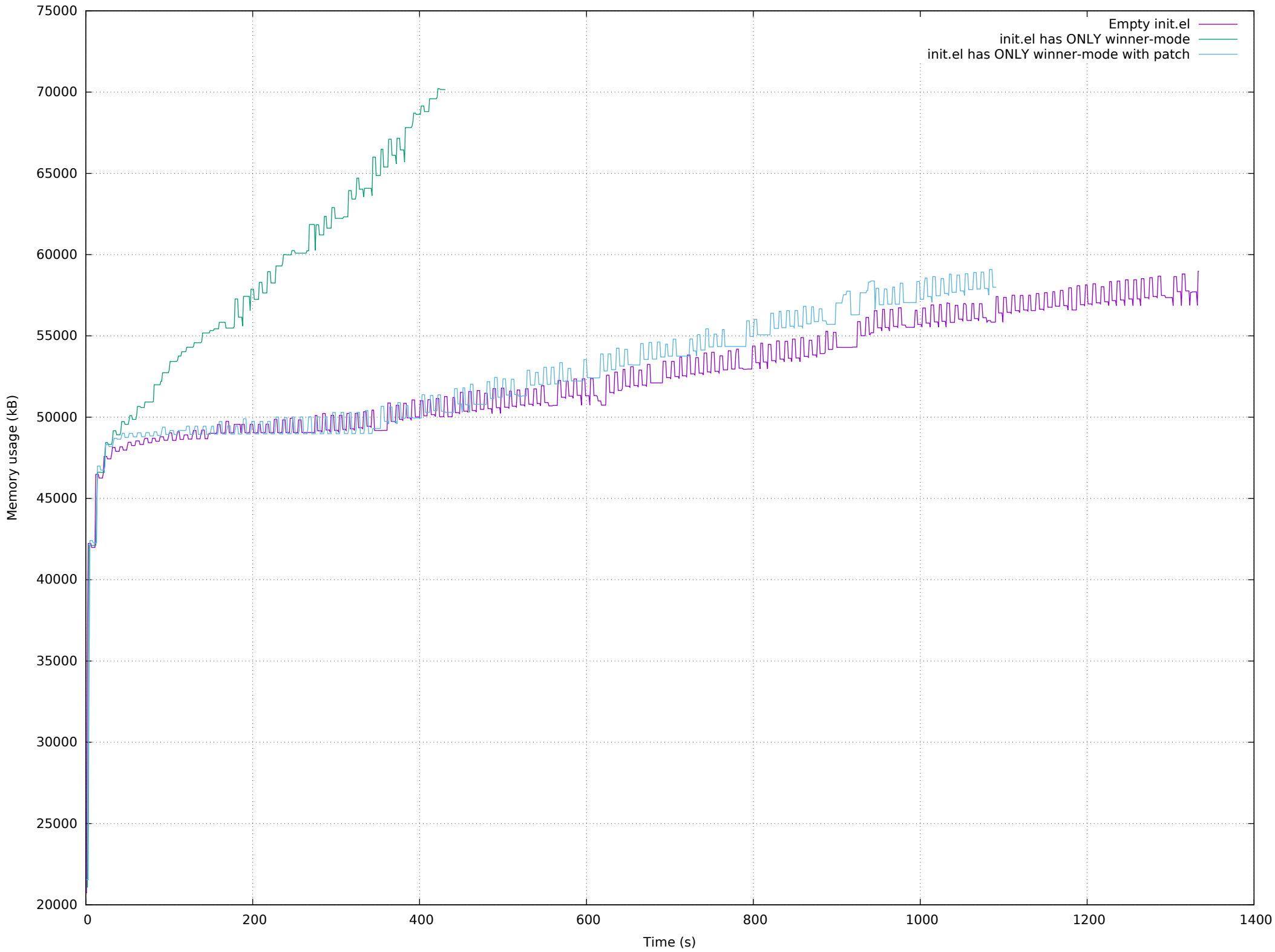
Emacs memory consumption as clients are created/destroyed
