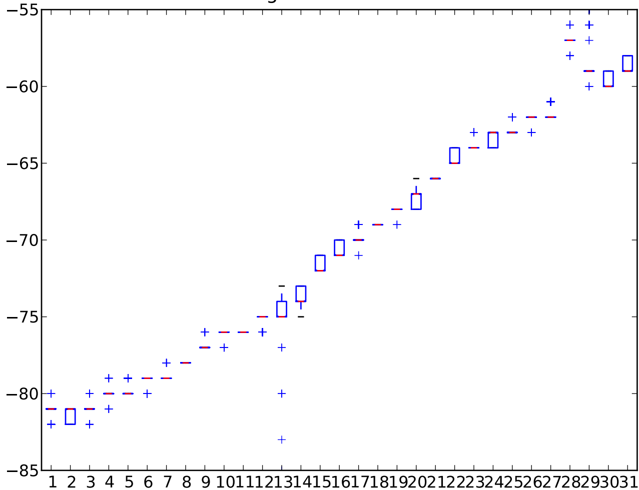
Average RSSI value in dBm
