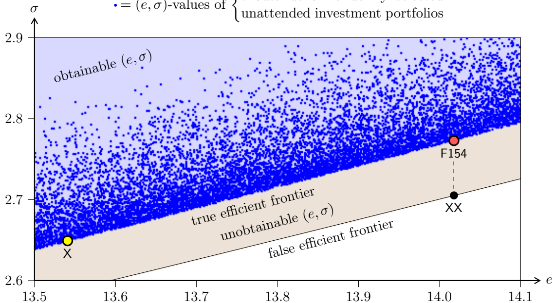
Figure 1: Near the efficient boundary in the e\sigma -plane
